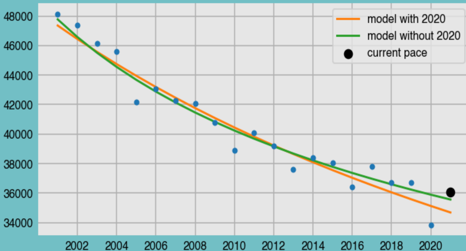
2021 Deaths using Mortality Rate of each Year
